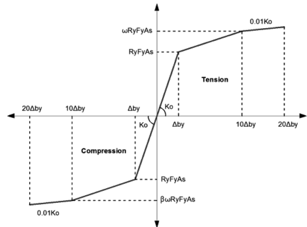
Figure 1. Assumed backbone curve for buckling-restrained braces.
