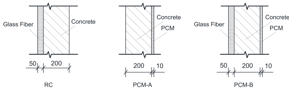
Figure 5. Constructions of the three configurations (Unit: mm).
