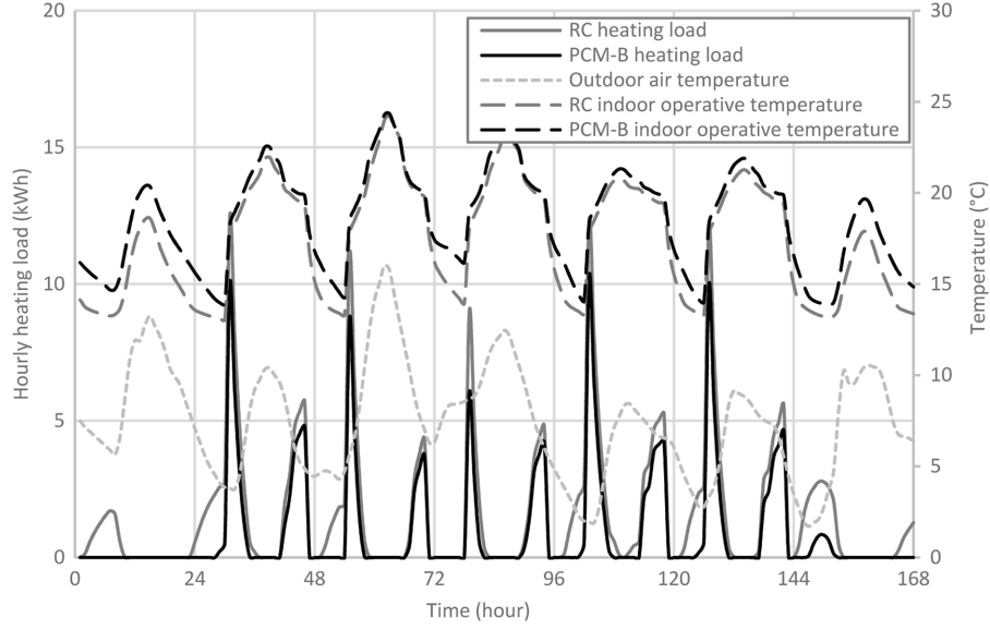
Figure 11. Hourly heating load and indoor operative temperature of RC and PCM-B ( T_M = 22^\circ\text{C} ) for a south-oriented cellular office room with WWR = 40% in Dec 3-9.
