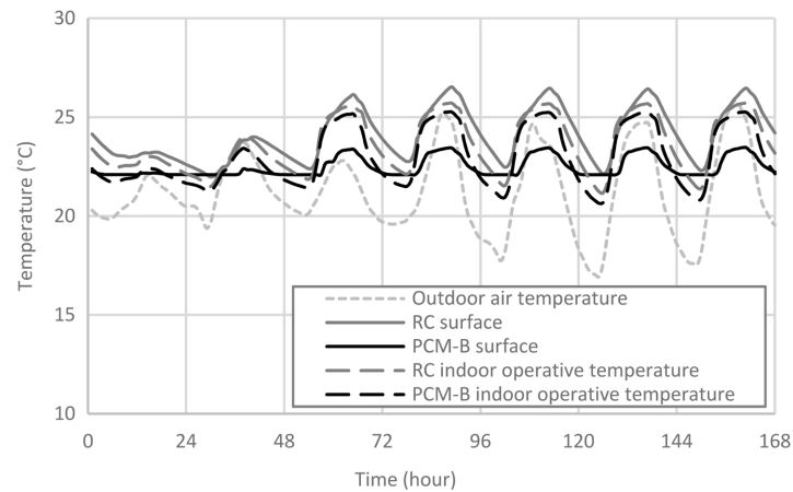
Figure 8. Comparison of the façade inner surface temperature and indoor operative temperature of RC and PCM-B ( T_M = 22^\circ\text{C} ) for a south-oriented cellular office room with WWR = 40% from June 3-9.
