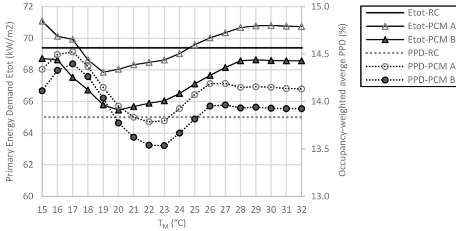
Figure 6. Primary energy demand and occupancy-weighted average PPD vs. T_M for RC, PCM-A, and PCM-B for a south-oriented cellular office room with WWR = 40%.
