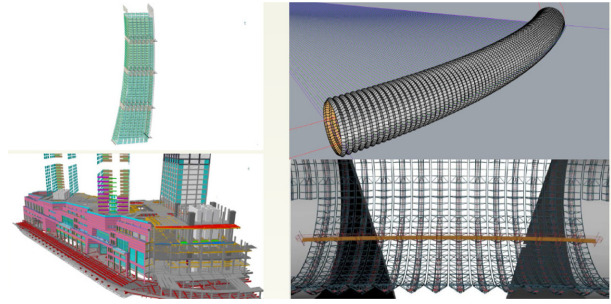
Figure 11. Multi-dimensional façade-structure integration.
