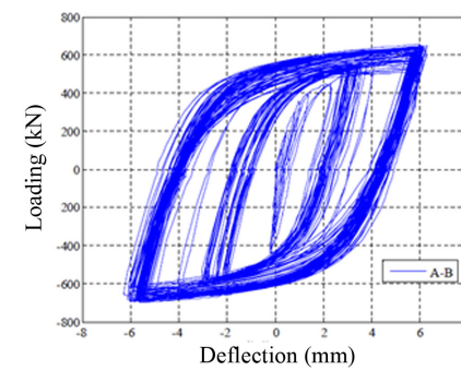
(a) Physical test
