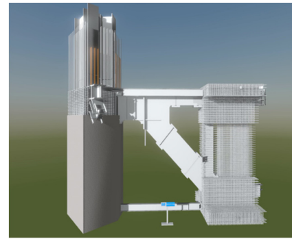
(a) Hybrid outrigger
