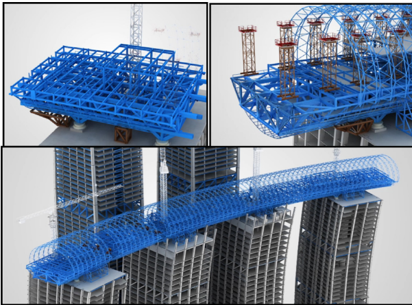
Figure 10. Horizontal construction simulation for conservatory.
