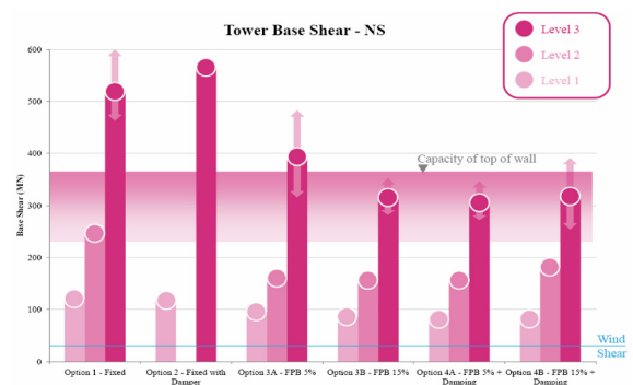
(b) Effectiveness of mass damping
