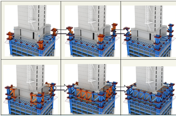
Figure 9. Vertical erection simulation for towers.
