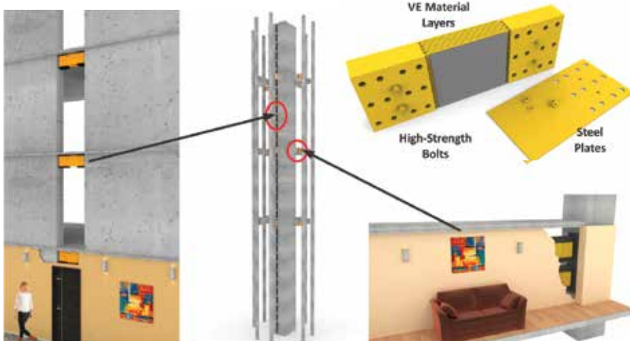
Figure 22. The Viscoelastic Coupling Damper (VCD) can be inserted into party walls, so as to avoid obstructing leasable space. © Kinetica
