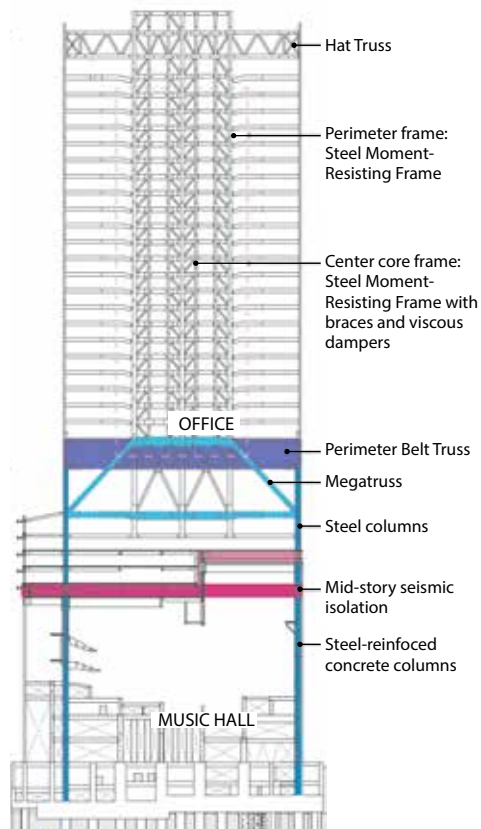
Figure 19. Diagram of seismic isolation strategy used for Nakanoshima Festival Tower, Osaka. © Nikken Sekkei
