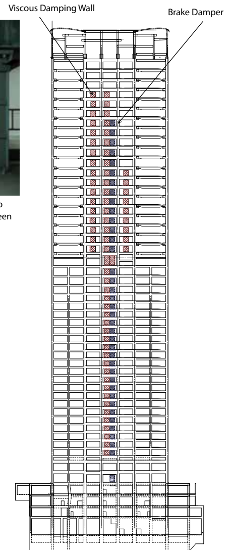
Figure 17. Section showing location of damping equipment at Ark Hills Sengokuyama Mori Tower, Tokyo. © Obayashi Corporation
