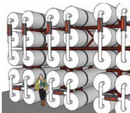
Figure 21. The Hummingbird is a tuned liquid-column gas damper, which can be easily distributed throughout a building. © Hummingbird Kinetics
