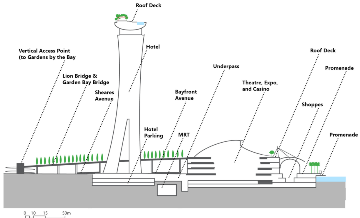
Figure 2. Marina Bay Sands Section (Credit: Anna Kleinsasser).
