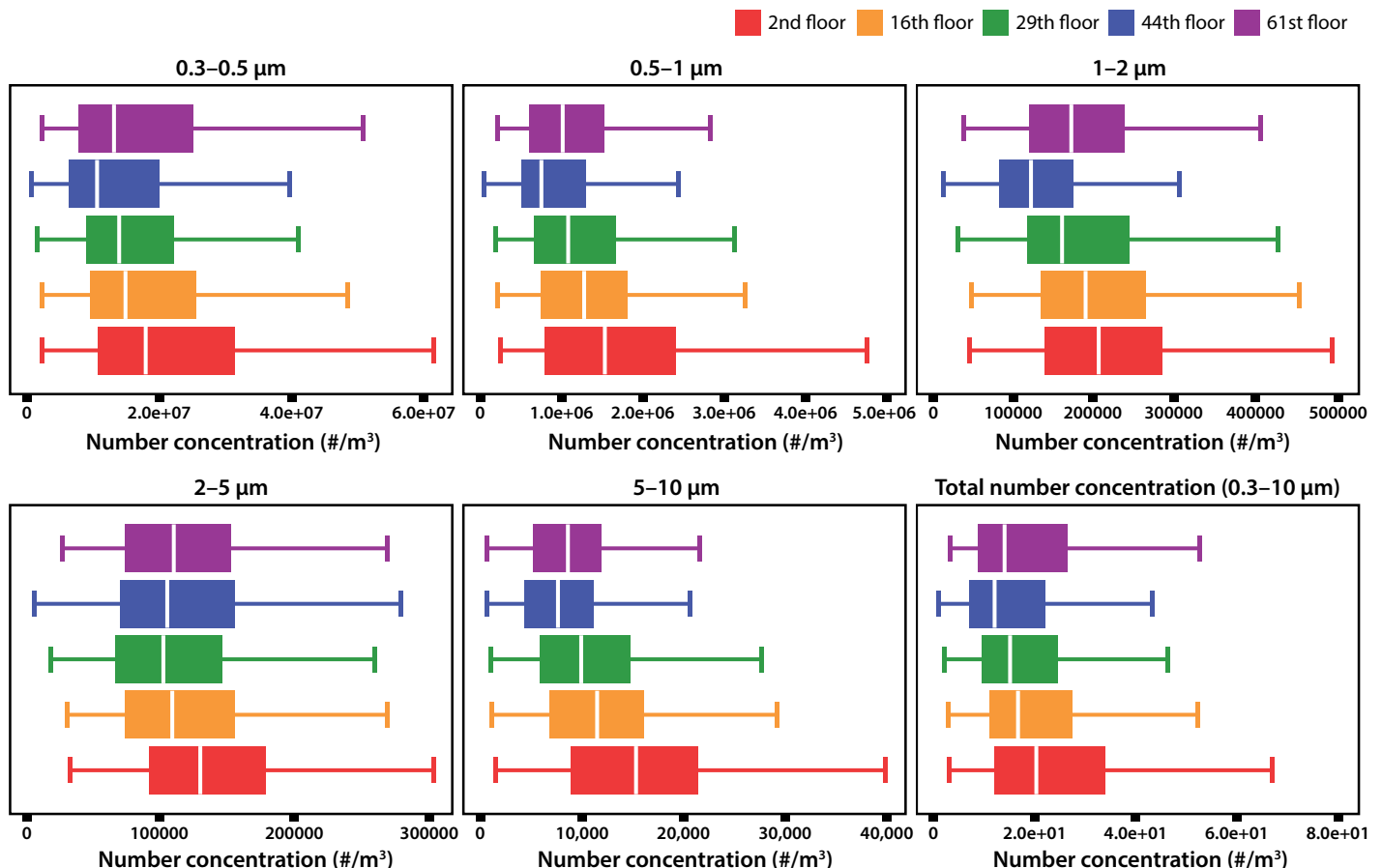
Figure 3. Box plots of size-resolved particle number concentration data measured on each of the five floors. Bins include: 0.3–0.5 μm, 0.5–1 μm, 1–2 μm, 2–5 μm, 5–10 μm, and total number concentrations (0.3–10 μm). Outliers are excluded for graphical clarity.
