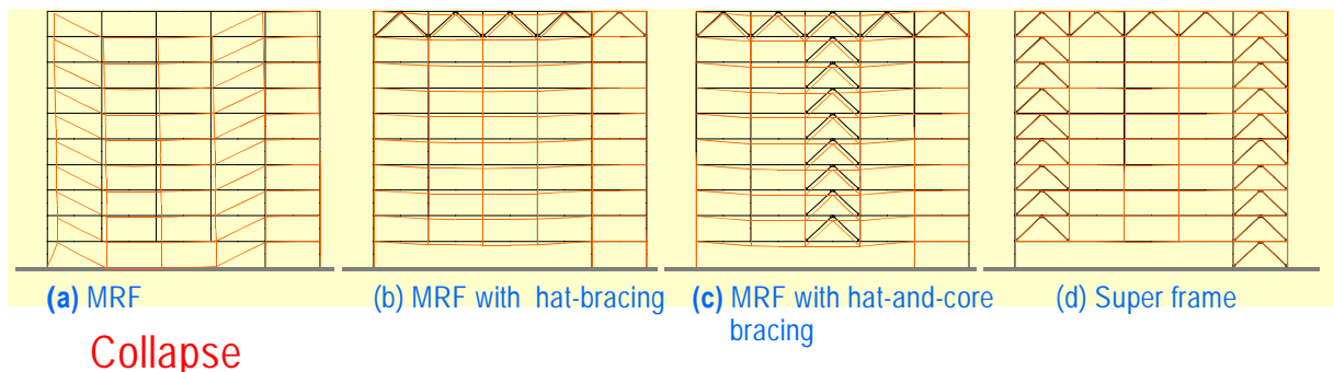
Fig. 5. Analysis Results for Various Frame Systems at Time of Column Loss
