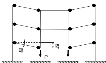
Fig. 7. Simple Assessment of the Vertical Load Supporting Capacity of Beams
