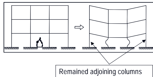
Fig. 8. Assessment of the Loading Capacity of Remaining Adjacent Columns
