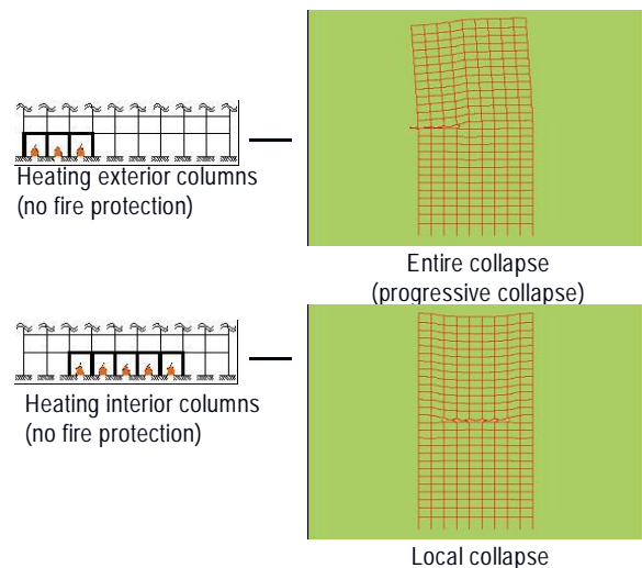
Fig. 6. Analysis Results for Thermal Elasto-Plasticity and Buckling during Fire
