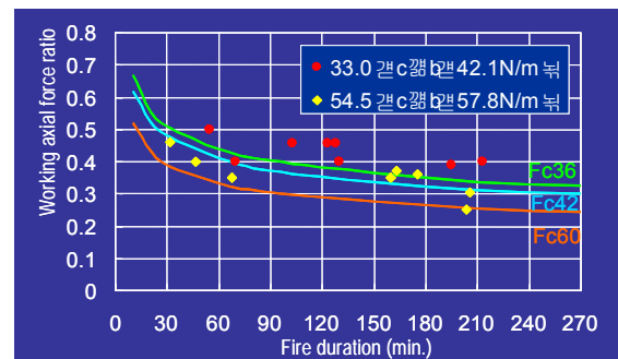
Fig. 10. Heated Loading Test Results for Unprotected CFT Column
