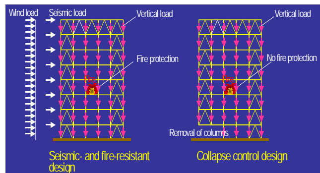
Fig. 2. Image of Collapse Control Design.
