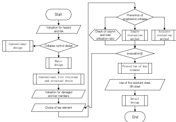
Fig. 3. Outline of Recommended Flow of Collapse Control Design
