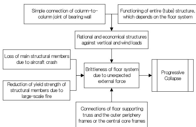
Fig. 1. Analysis of Causes of WTC Collapse.
