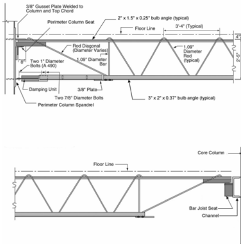
Figure 4 Steel truss details
