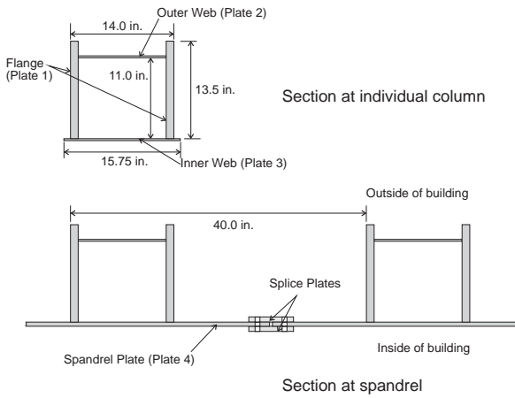
Figure 3 Cross section of exterior column
