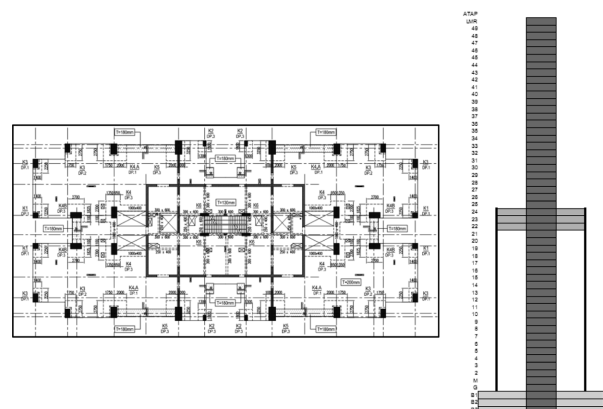
Figure 2. Structural plan and cross section.
