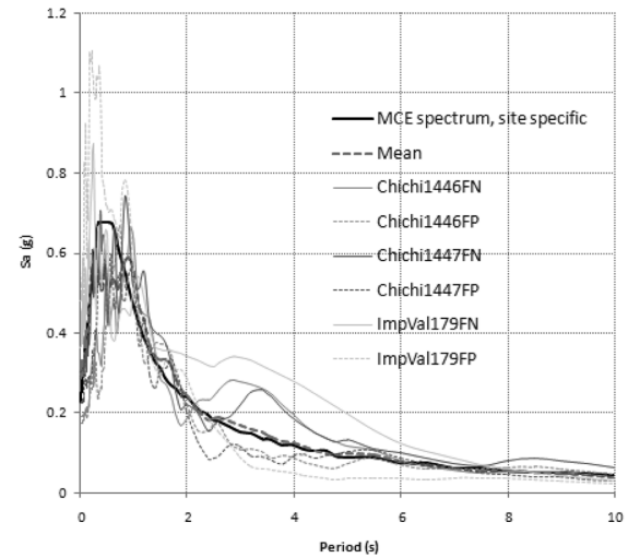
Figure 4. NLRHA target spectrum.
