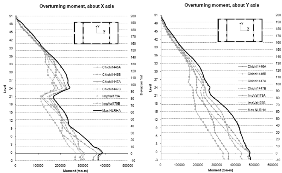
Figure 10. Overturning moment.
