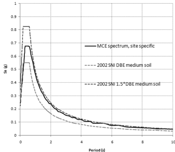
Figure 5. Comparison between NLRHA and RSA target spectrum.
