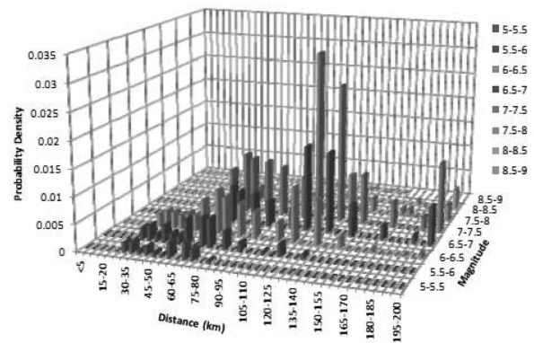
Figure 6. De-aggregation hazard result of 2500 year return period for Jakarta, T = 0.2 sec (Hendriawan & Azis, 2010).
