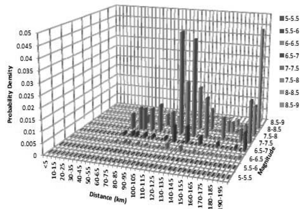
Figure 7. De-aggregation hazard result of 2500 year return period for Jakarta, T = 4.0 sec (Hendriawan & Azis, 2010).
