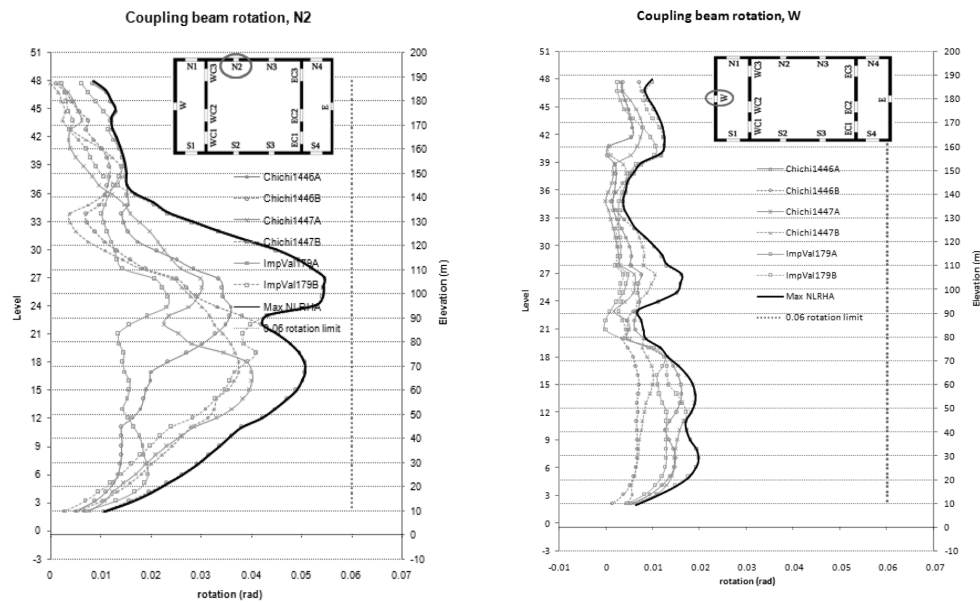
Figure 14. Coupling beam rotations.
