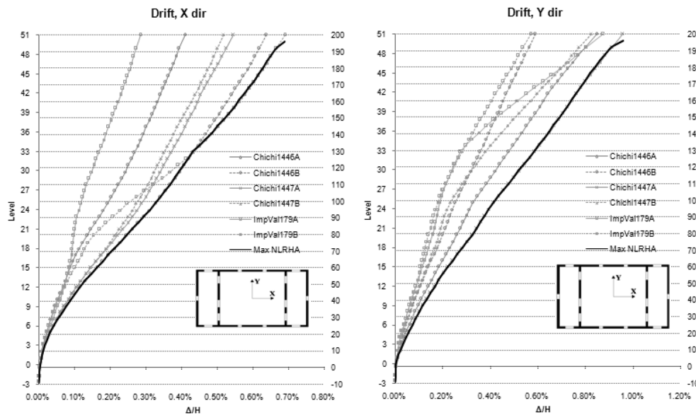
Figure 12. Maximum drift.
