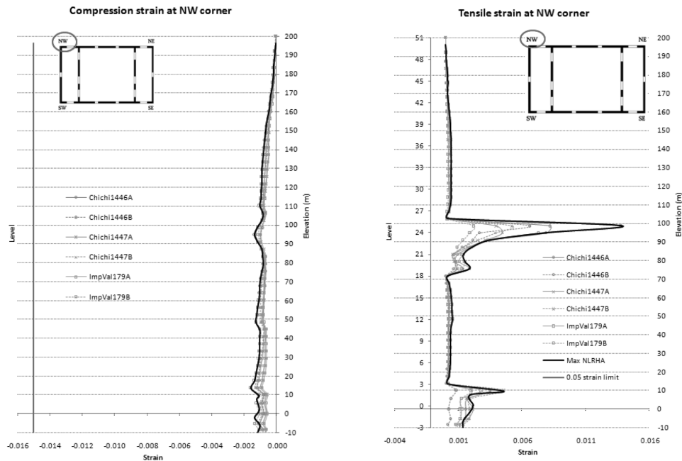
Figure 13. Core wall strains at Northwest corner.
