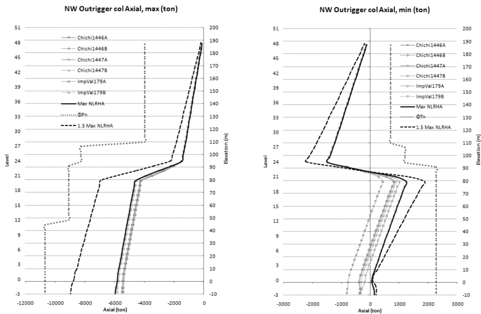
Figure 16. Outrigger column axial.
