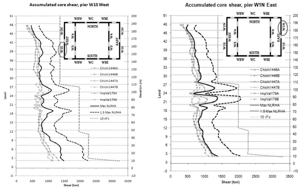
Figure 15. Individual core wall pier accumulated shear.
