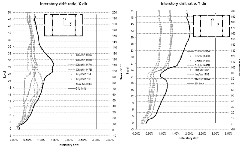
Figure 11. Maximum interstory drift.
