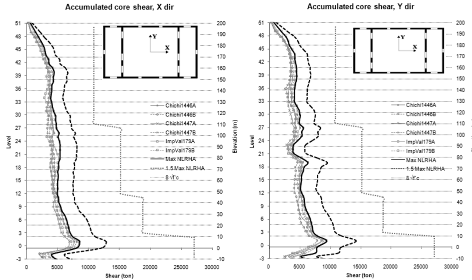
Figure 9. Core wall accumulated shear.
