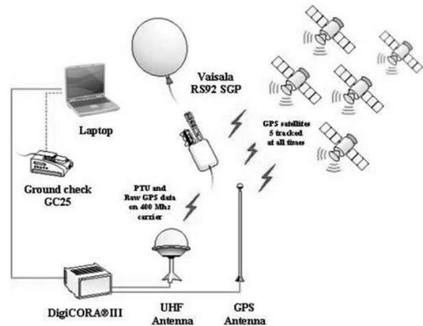
Figure 1. Radiosonde system.
