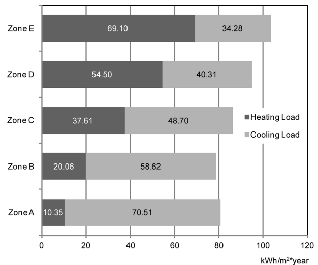
Figure 4. Annual heating and cooling loads of perimeter zone.
