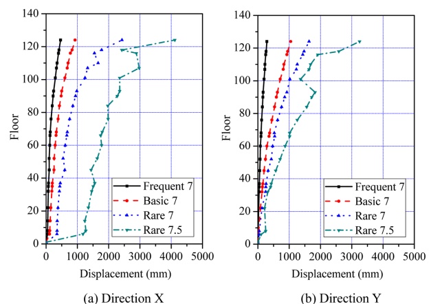
Figure 5. Maximum floor displacement.
