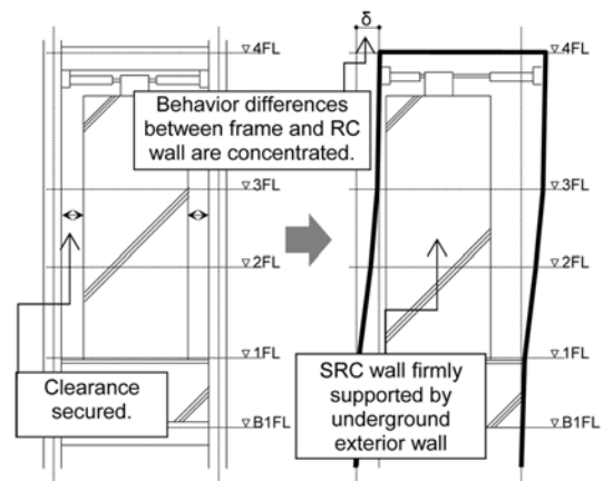
Figure 15. Illustrated concept of Big Wall Frame.
