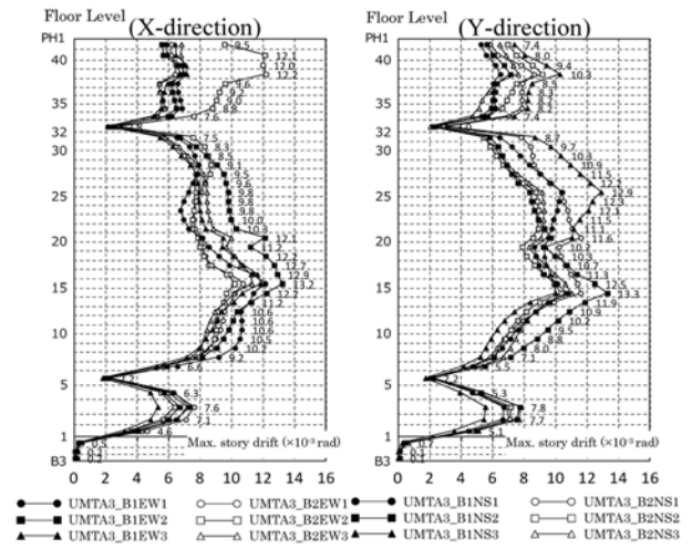
Figure 21. Results of seismic response analysis, Daishinken Wave 3B (max. story drifts).
