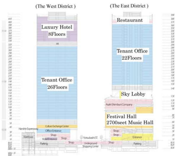
Figure 3. Sectional view of both West and East Districts.
