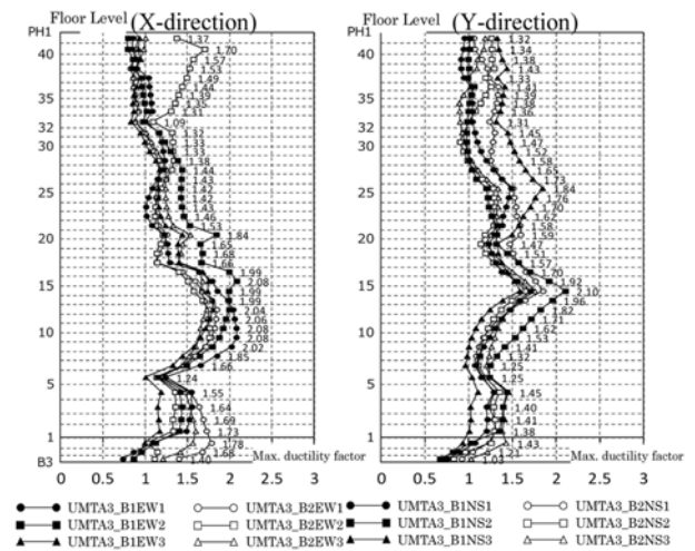
Figure 22. Results of seismic response analysis, Daishinken Wave 3B (max. ductility factors).
