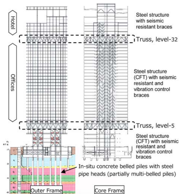
Figure 9. Sectional view of framing structure.
