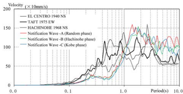
Figure 17. Velocity response spectra (Level 2 and h = 0.05 ).
