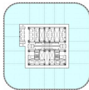
Figure 6. Typical low-rise office floor plan.
