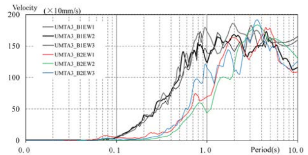
Figure 18. Velocity response spectra (Daishinken Wave 3B (EW direction), h = 0.05 ).
