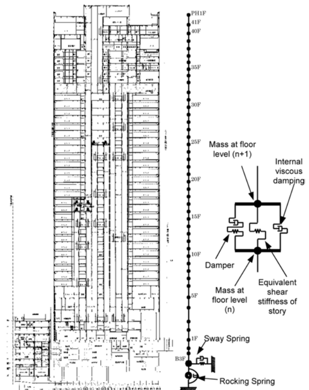
Figure 16. Illustrated analysis model.
