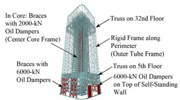
Figure 7. Rendering of framing structure.
