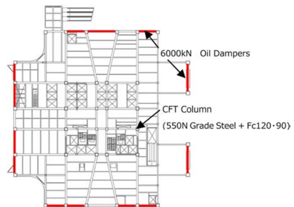
Figure 11. Framing plan, level 3.
