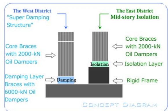
Figure 8. Concept diagram of structural planning.
