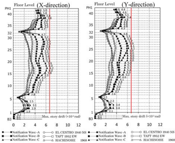
Figure 19. Results of seismic response analysis, Level-2 (max. story drifts).
