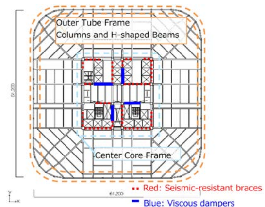
Figure 10. Typical floor framing plan.
