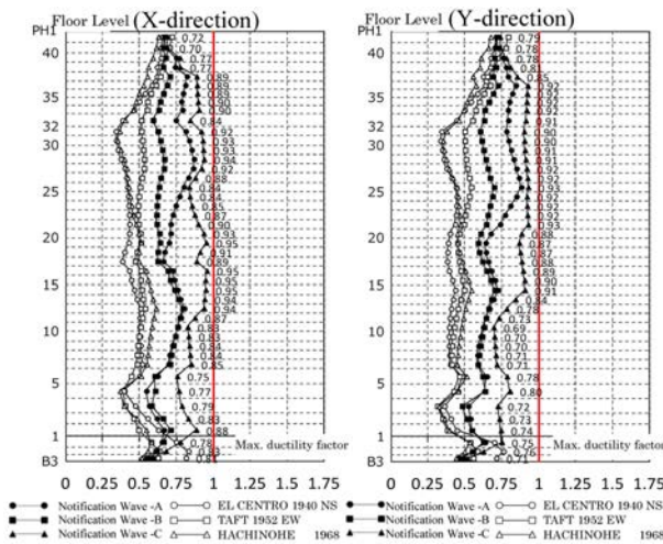
Figure 20. Results of seismic response analysis, Level-2 (max. ductility factors).
