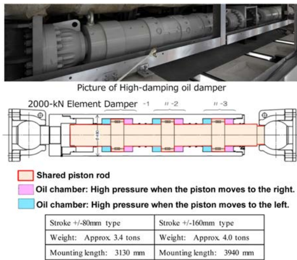
Figure 12. High-damping oil damper.
