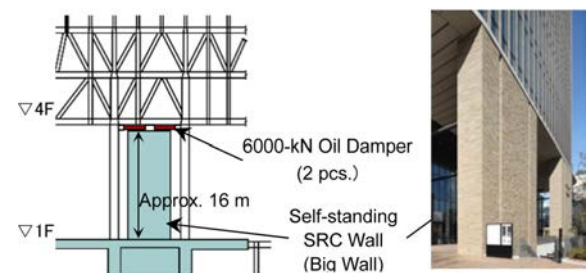
Figure 14. East framing elevation.
