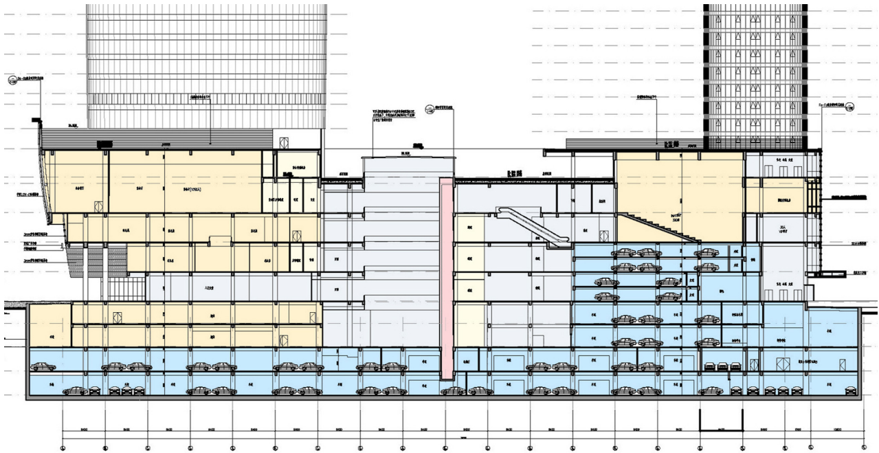
Figure 14. The multi-level parking lot within and below the podium.
