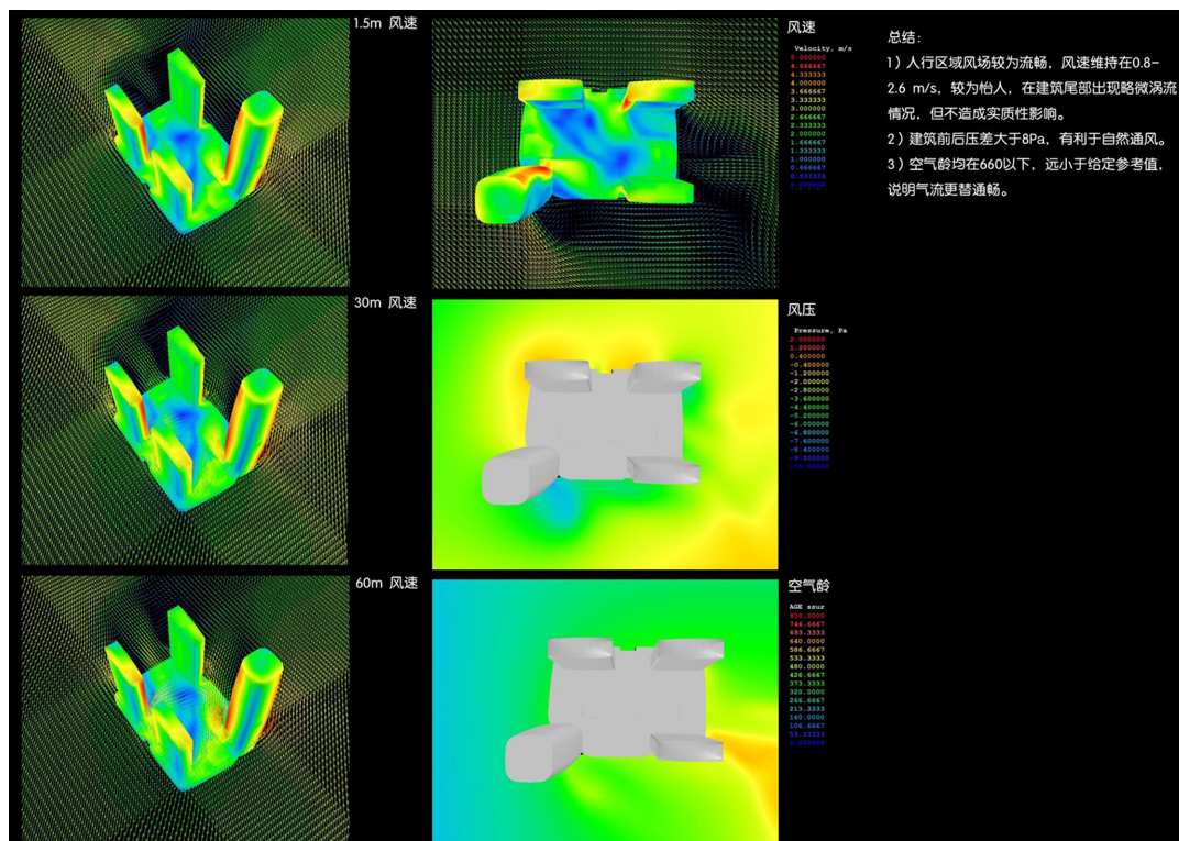
Figure 15. The wind simulation of the complex.
