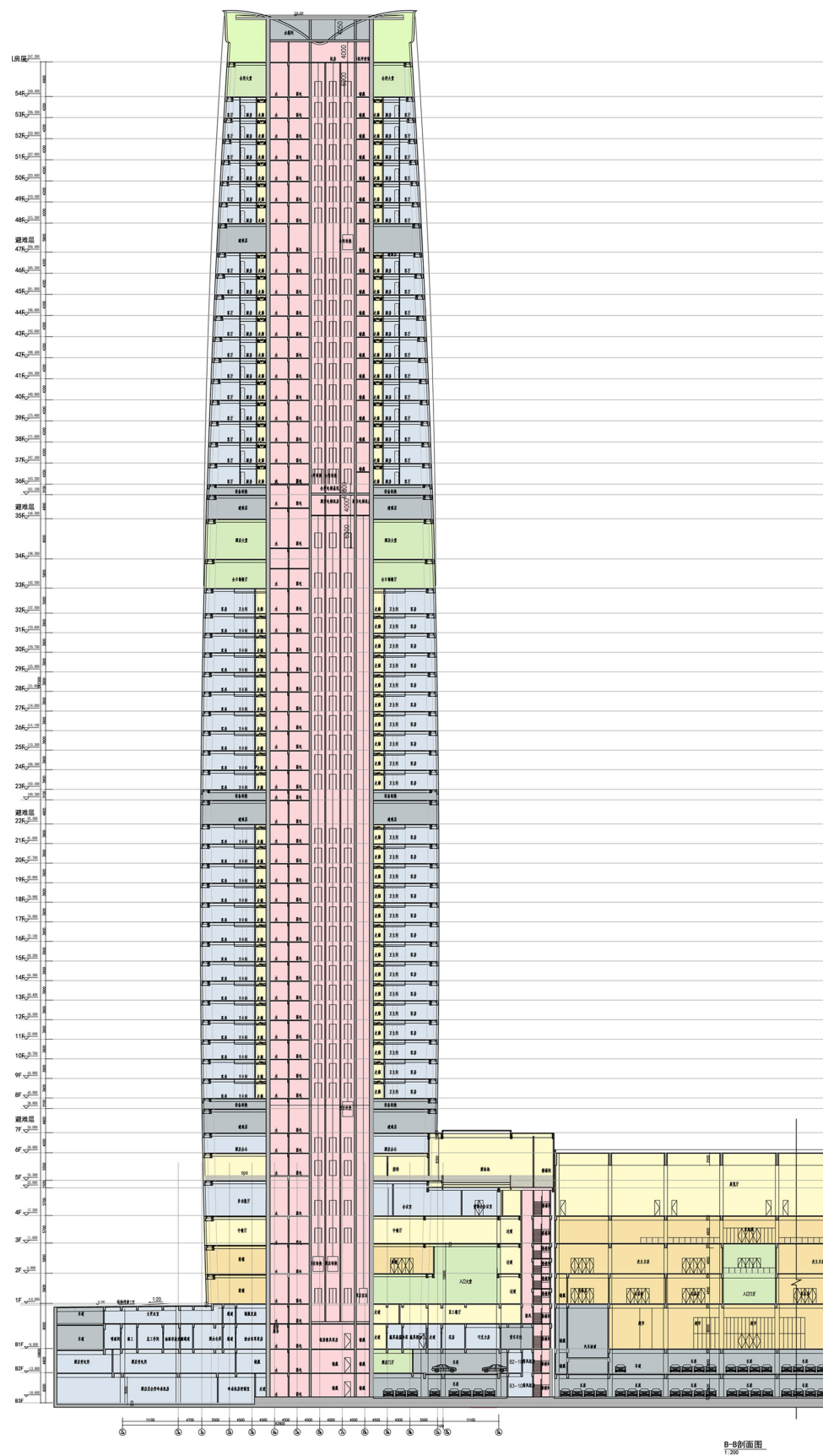
Figure 10. The three-dimensional and multi-functional layout of the main building.
