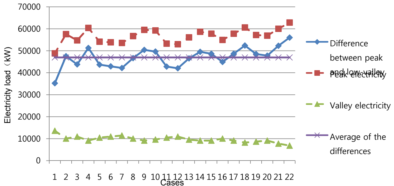
Figure 9 Peak to valley difference in electricity load on the typical summer day
