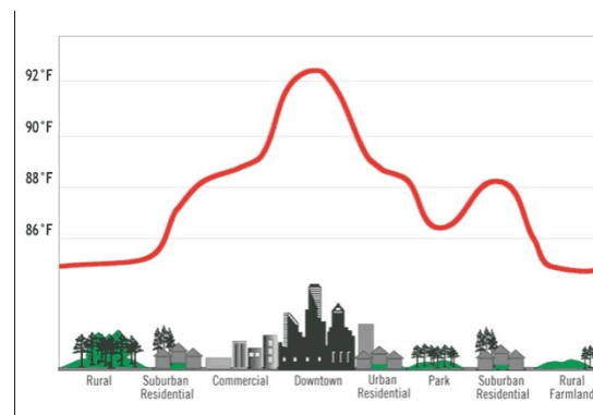
Figure 1 The schematic of heat island effect (EPA, 2011)
