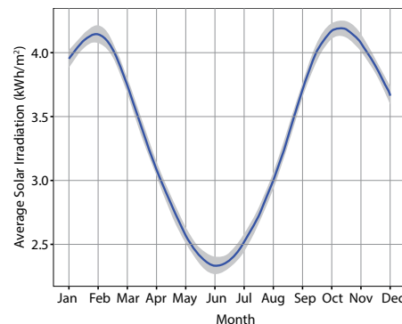
Figure 5. Average solar irradiation (kWh/m²) by month.
