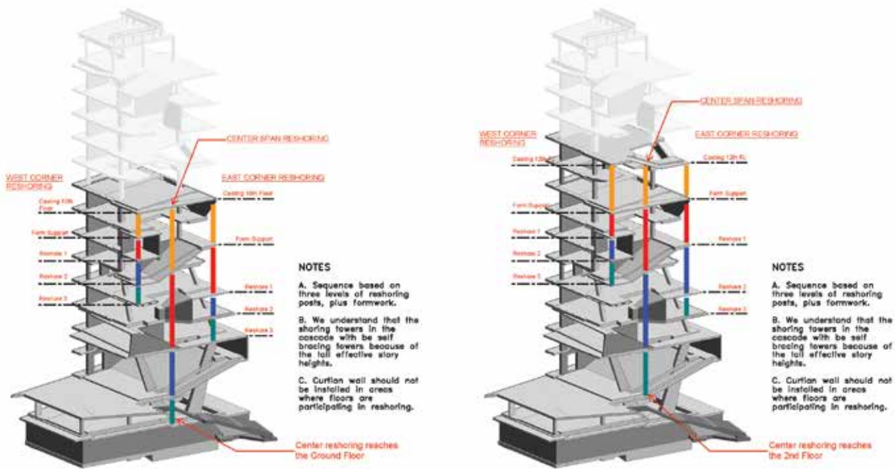
Figure 5. Due to variation in support arrangements of the Cascade, concrete reshoring requirements varied along the south façade of the building (Source: Diller Scofidio + Renfro)
