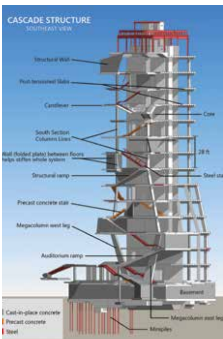
Figure 11. Overview of the structural components of the Cascade (Source: Leslie E. Robertson Associates)
