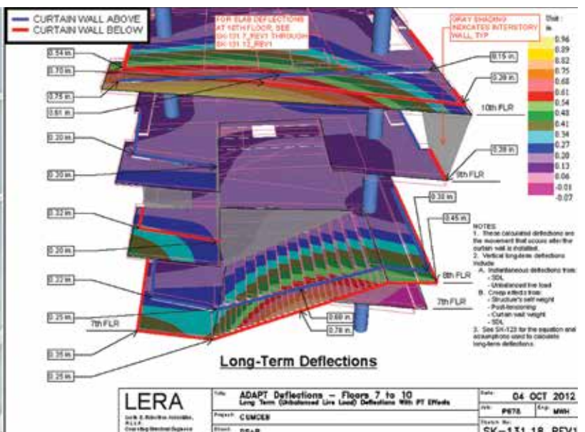
Figure 9. The cantilevered slab performance was coordinated by "neighborhood", here in Floors 7 through 10, with the façade system requirements during a design assist process with the Curtain Wall Contractor (Source: Diller Scofidio + Renfro left / Leslie E. Robertson Associates)
