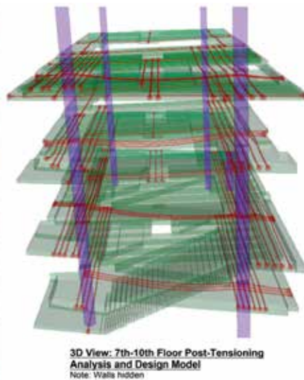
Figure 8. Bonded post-tensioning system as idealized during structural analysis and as constructed (Source: Columbia University Left / Leslie E. Robertson Associates)
