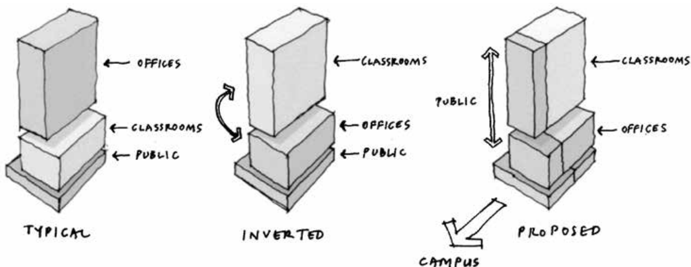
Figure 2. Building massing diagram identifying the vertical arrangement of public space on the campus-facing south façade, defining the "Study Cascade". (Source: Diller Scofidio + Renfro)
