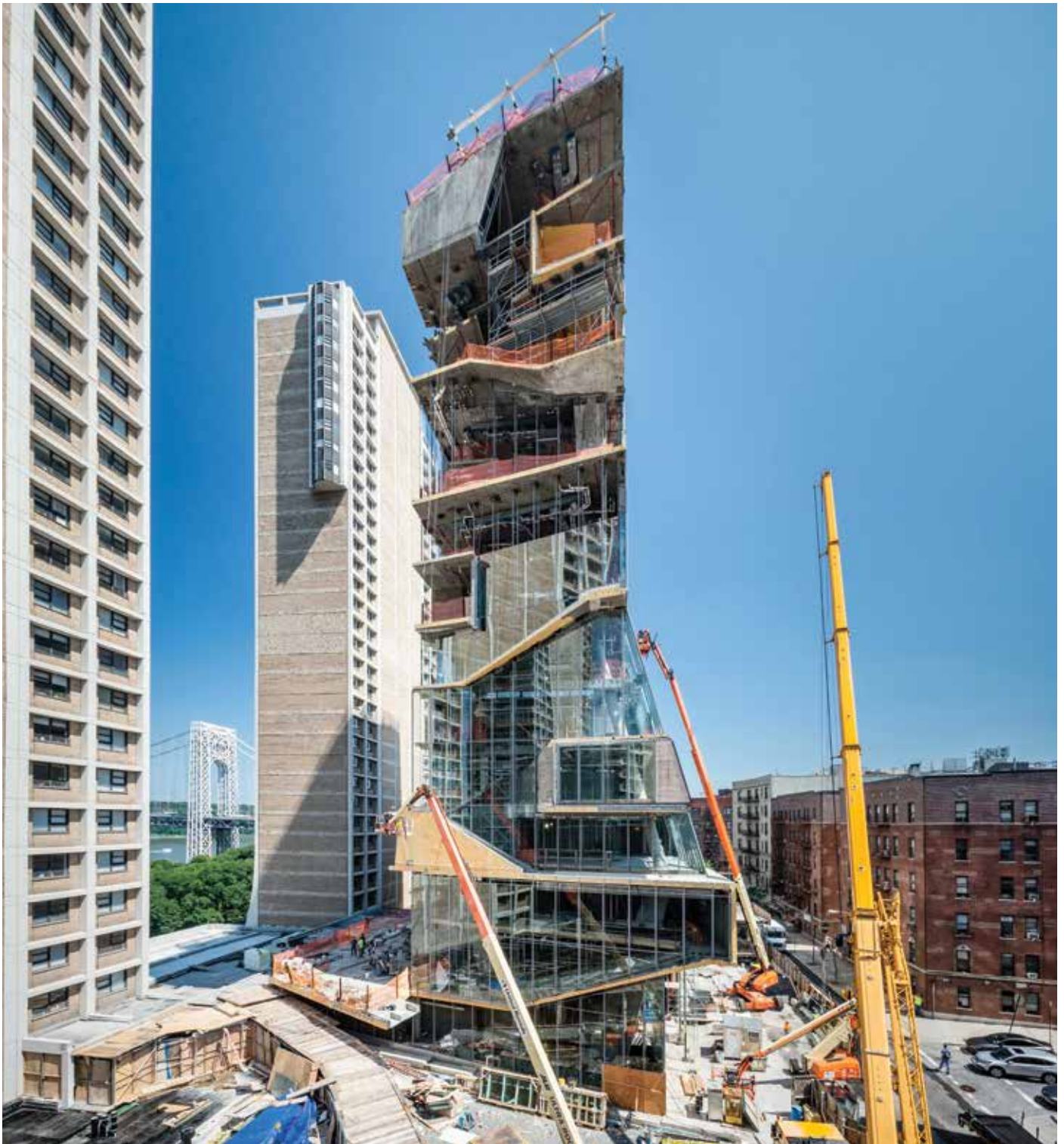
Figure 15. Current progress and neighborhood (Source: Leslie E. Robertson Associates)
