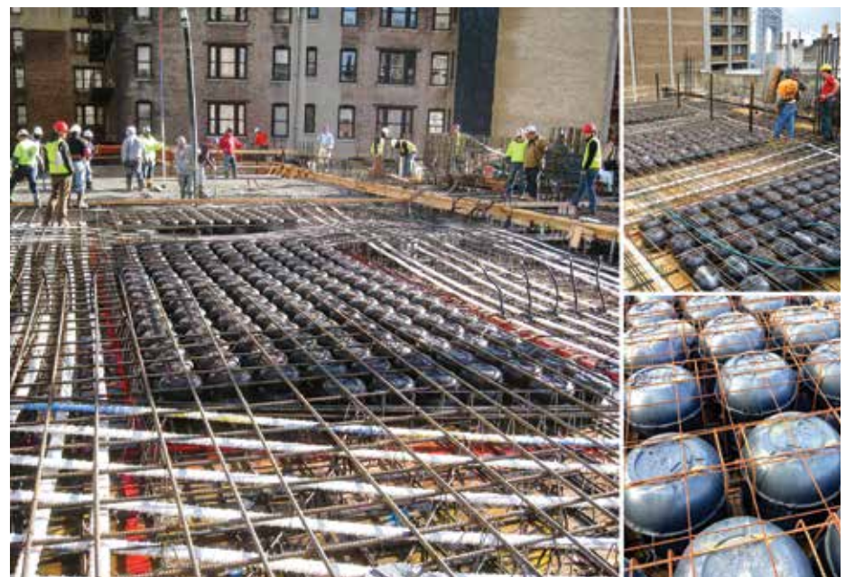
Figure 7. Construction materials: slab void formers placed between bands of bonded post-tensioning (Source: Matthew Melrose)
